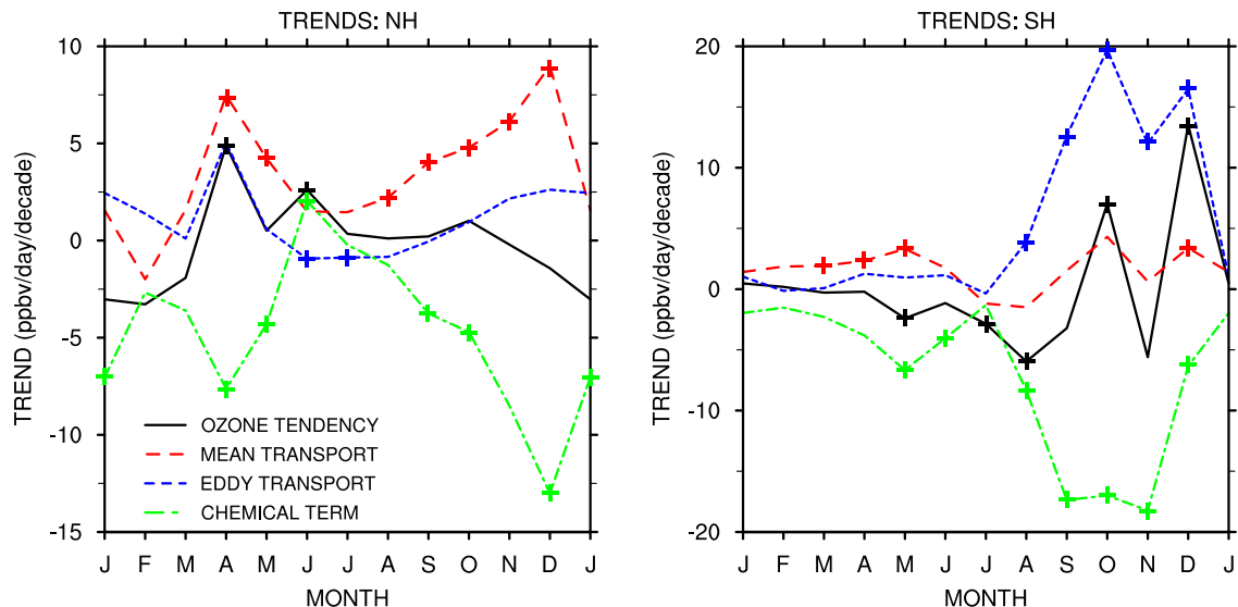
Figure 6. Annual cycle of the trends in the ozone tendency and its forcing terms, for the (left) NH and the (right) SH. The trends are calculated after the zonal-mean ozone tendency and its forcing terms are averaged between 100 and 20 hPa and between 60^\circ – 85^\circ . Trends that are statistically significant at the 95% statistical significance level are indicated by a cross.
