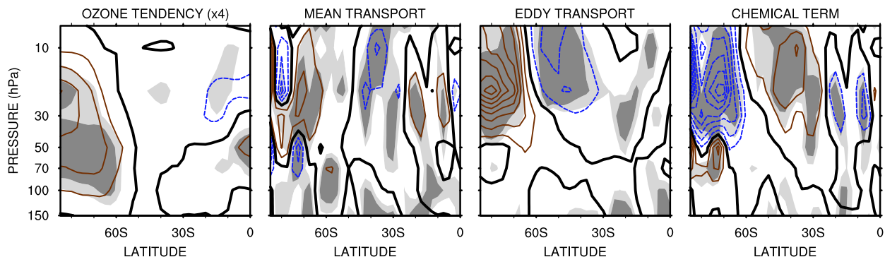
Figure 7. OND trends in the ozone tendency and its forcing terms for the SH. Dashed blue (solid brown) lines represent negative (positive) values while the bold solid line represents the zero-line. Light grey (dark grey) shading represents the 95% (99%) statistical significance level of the trends. Contour spacing is 10 \text{ ppbv day}^{-1} per decade. Note that the trends in the ozone tendency are weak compared to the forcings terms and are therefore multiplied by 4.
