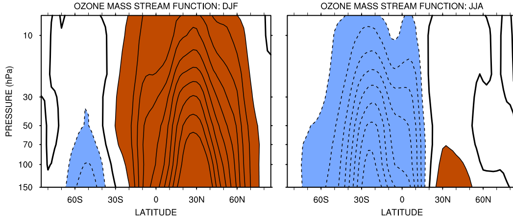
Figure 3. Ozone mass stream function associated with the Brewer-Dobson circulation averaged over (left) DJF and (right) JJA 1980-2001. Blue (brown) colors with dashed (solid) white lines represent negative (positive) values while the bold solid line represents the zero-line. Contour spacing is 10^3 \text{ kg s}^{-1} .
