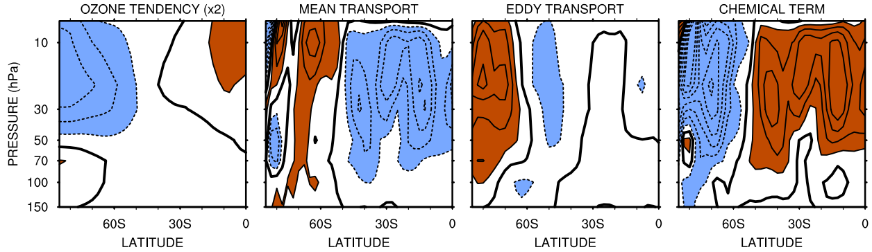
Figure 2. Zonal-mean ozone tendency and its forcing terms averaged over DJF 1980-2001 in the SH. Dashed (solid) lines and blue (brown) colors represent negative (positive) values while the bold solid line represents the zero-line. Contour spacing is 10 \text{ ppbv day}^{-1} . Note that the ozone tendency is weak compared to its forcing terms and is therefore multiplied by 2.
