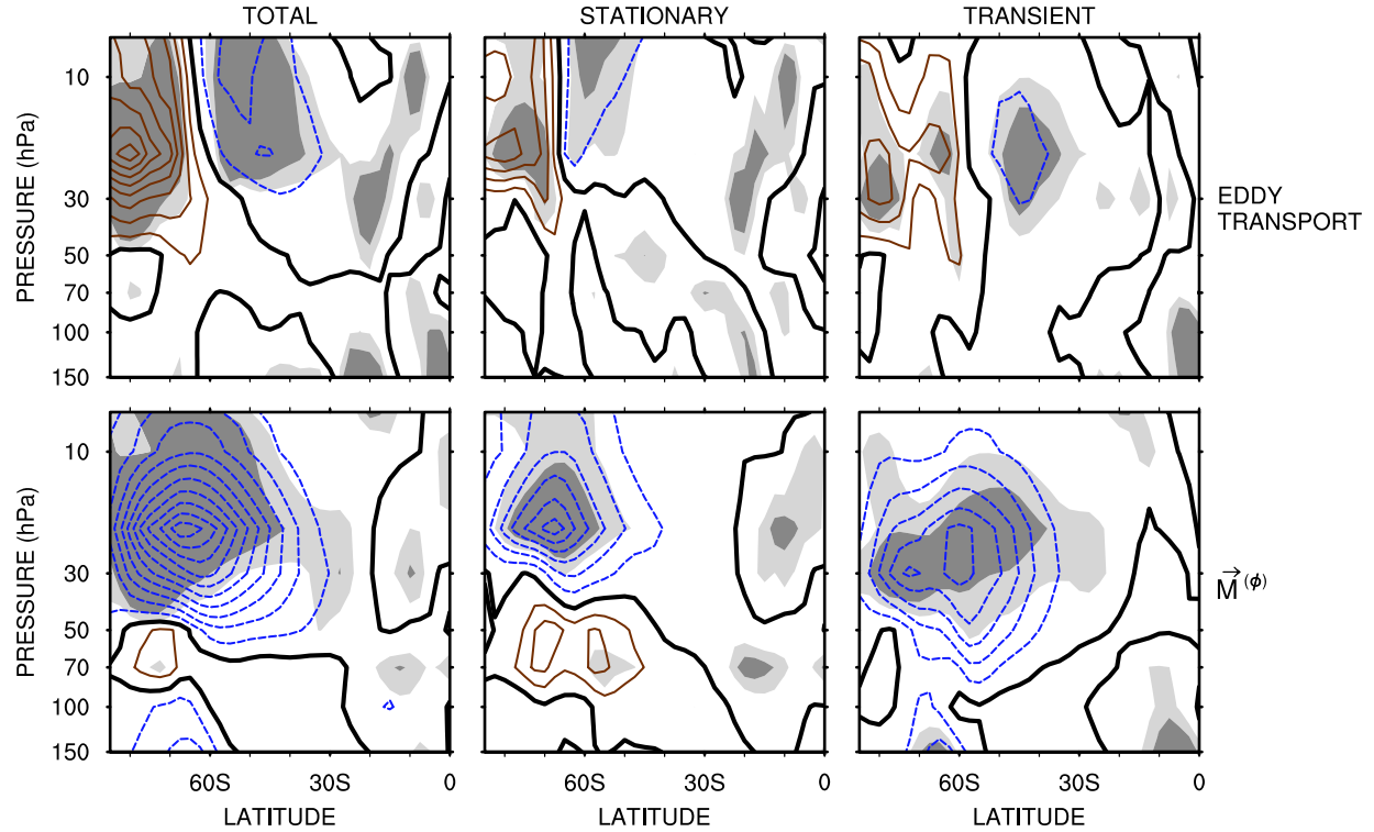
Figure 8. Same as Figure 7 but for the eddy ozone transport and the horizontal component of the eddy ux vector, with the contributions of stationary and transient waves. Contour spacing is 10 \text{ ppbv day}^{-1} per decade for the eddy transport and 2 \times 10^5 \text{ kg ppbv m}^{-2} \text{ day}^{-1} per decade for \vec{M}^{(\phi)} .
