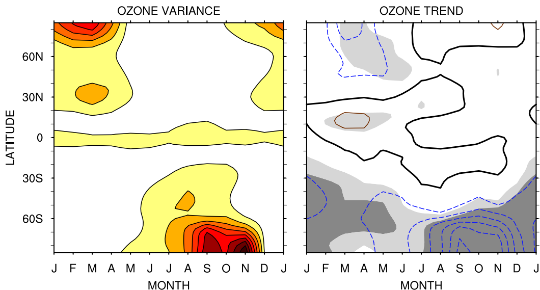
Figure 5. Annual cycle of the ozone sample variance and trend. The variances and trends are calculated after the zonal-mean ozone is averaged between 100 and 20 hPa. Dashed blue (solid brown) lines represent negative (positive) values while the bold solid line represents the zero-line. Light grey (dark grey) shading represents the 90% (99%) statistical significance level of the trends. Contour spacing is 0.05 ppmv 2 for the ozone variance and 0.1 ppmv per decade for the ozone trend.
