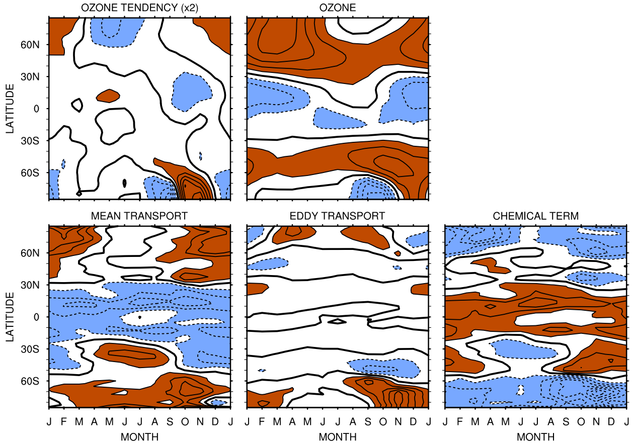
Figure 1. Annual cycle of the zonal-mean ozone, represented by the departures from the global mean (2 ppmv), and of the zonal-mean ozone tendency and its forcing terms, averaged between 100 and 20 hPa. Dashed (solid) lines and blue (brown) colors represent negative (positive) values while the bold solid line represents the zero-line. Contour spacing is 0.2 ppmv for the ozone and 10 ppbv day -1 for the ozone tendency and its forcing terms. Note that the ozone tendency is weak compared to its forcing terms and is therefore multiplied by 2.
