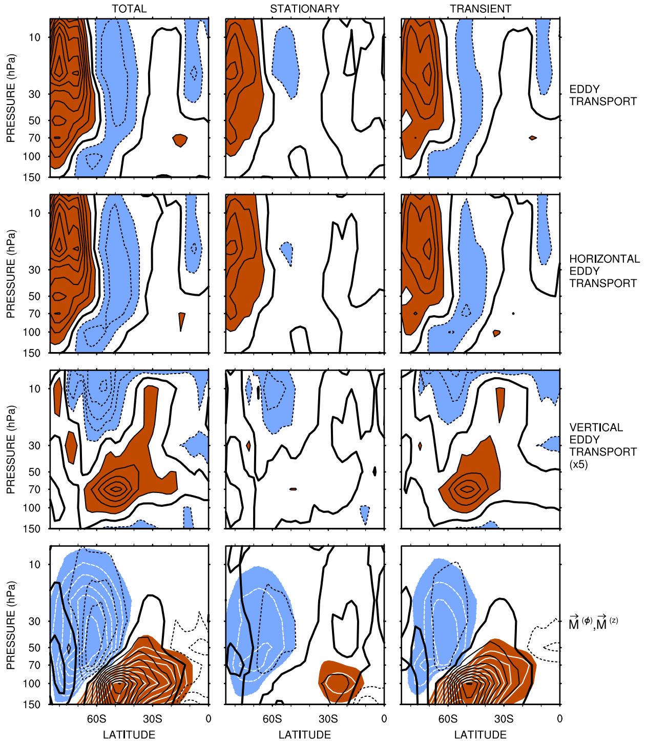
Figure 4. Same as Figure 2 but for the eddy ozone transport, its horizontal and vertical components, and the eddy ux vector, with the contributions of stationary and transient waves. Blue (brown) colors with dashed (solid) white lines represent negative (positive) values for \vec{M}^{(\phi)} . Dashed (solid) black lines represent negative (positive) values while the bold solid line represents the zero-line for \vec{M}^{(z)} . Contour spacing is 10 \text{ ppbv day}^{-1} for the eddy transport and its horizontal and vertical components, 2 \times 10^5 \text{ kg ppbv m}^{-2} \text{ day}^{-1} for \vec{M}^{(\phi)} and 2 \times 10^2 \text{ kg ppbv m}^{-2} \text{ day}^{-1} for \vec{M}^{(z)} . Note that the vertical eddy transport is weak compared to the horizontal eddy transport and is therefore multiplied by 5.
