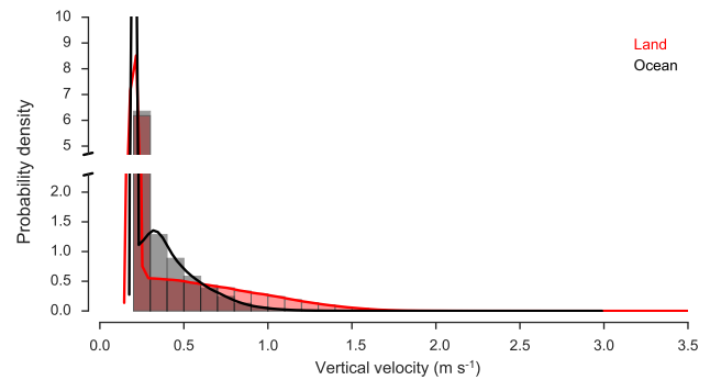
Figure 1. Distributions of model-predicted instantaneous subgrid-scale vertical velocity for near-surface (below 700 mb) grid cells broken down by land (red) and ocean (black) regimes.
