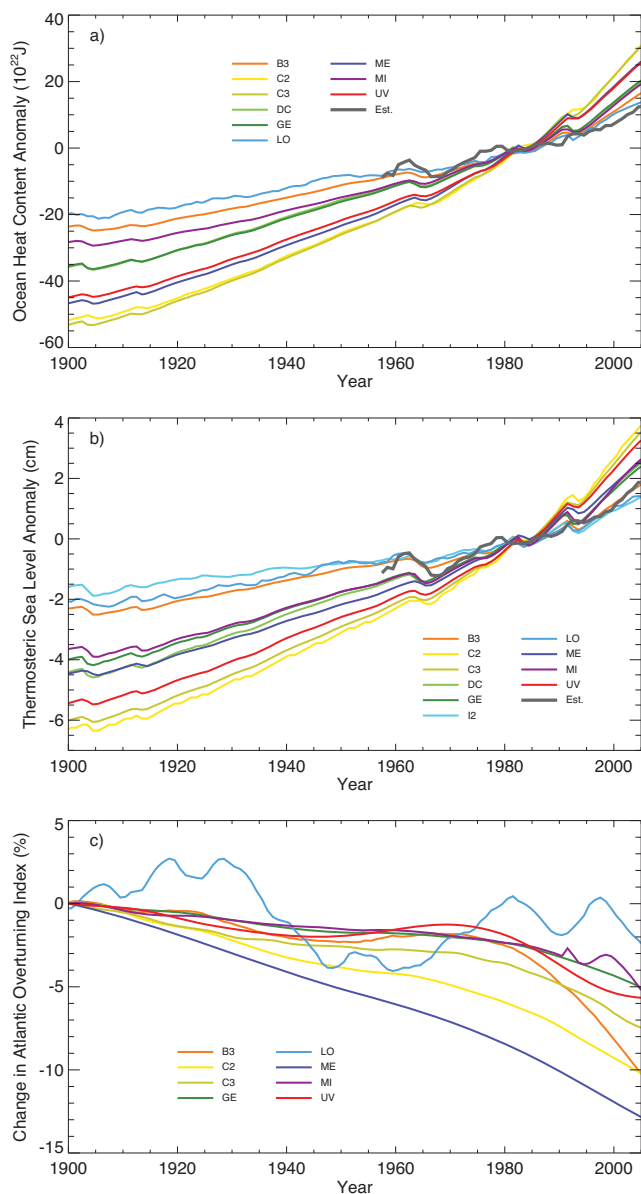
Fig. 3. Changes in global ocean heat content (a), thermosteric sea level rise (b), and North Atlantic overturning index (c) over the last century. The dark grey lines are estimates of the change in heat content (a), and the thermosteric component of sea level change (b), of the first 2000 m of the ocean, from Levitus et al. (2012). Ocean heat content (a) and thermosteric sea level (b) are plotted as anomalies from the year 1957 to 2005 average. Note that the model heat content and sea level changes are averages over the entire ocean so these would be expected to be somewhat larger than the values estimated over the first 2000 m. The North Atlantic overturning index (c) is shown as a percent change from the decade centred at year 1900 and was processed with a 30 yr moving average, rectangular filter.
