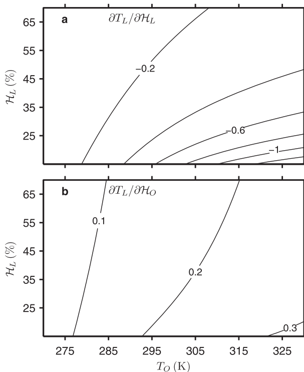
FIG. 3. Theoretical values for the partial derivatives of land surface air temperature with respect to (a) surface relative humidity over land ( \partial T_L/\partial H_L ) and (b) surface relative humidity over ocean ( \partial T_L/\partial H_O ) as a function of land relative humidity and ocean temperature [contour interval 0.2 \text{ K } \%^{-1} in (a) and 0.1 \text{ K } \%^{-1} in (b)]. Surface relative humidity over ocean is fixed at 80%. The partial derivatives are calculated by numerically solving the equal equivalent potential temperature Eq. (1).
