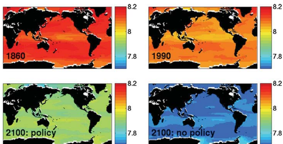
Fig. 4 Simulations of changes to the surface ocean pH (lower pH indicates a more acidic ocean) using the IGSM with a 3-dimensional ocean with biogeochemistry. Runs reflect business-as-usual (no policy) versus policy-restricted emissions scenarios, using a specified middle-of-the-road choice for climate sensitivity (approx. 2.3 K). The year 2100 atmospheric CO 2 concentration for these two runs was 558 ppmv (policy) and 928 ppmv (no policy)
