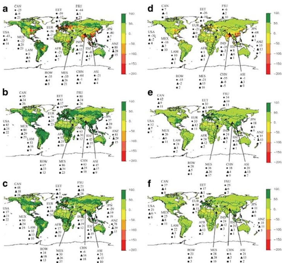
Fig. 3 Change in yield between 2000 and 2100 (gC/m 2 /year). Regional level percent changes in yield (crops) and NPP (pasture, forestry): Black circle —crops, Black triangle —pasture, Black square —forestry. a High Pollution scenario—no CO 2 or pollution controls. b Climate and GHGs only scenario—ozone damages removed c Capped pollution scenario—ozone precursors at 2000 levels d GHGs capped scenario—consistent with 550 CO 2 -eq. stabilization e GHGs capped-no ozone scenario. f GHGs and pollution capped scenario. Source: Reilly, et al. 2007
